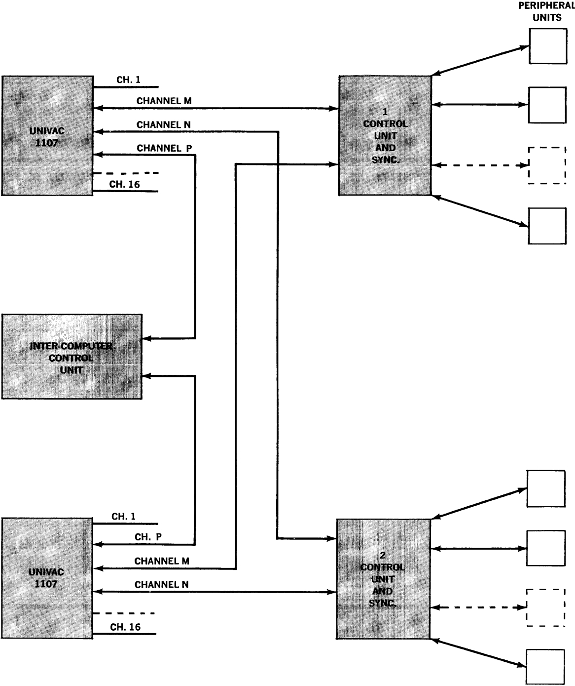
Figure 6-1. Two 1107 Computers Sharing the Same Peripheral Equipment and Communicating Directly with Each Other
